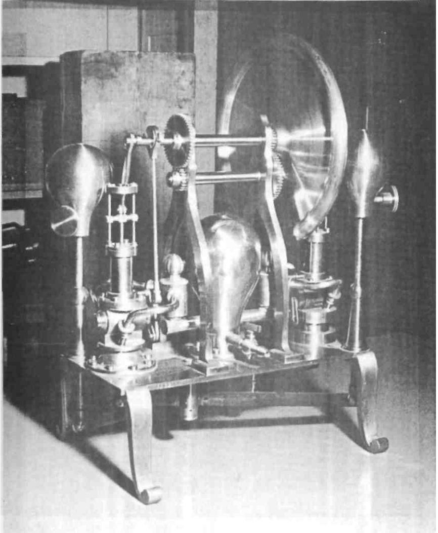
Hydro-Vacuo Motor or Engine
