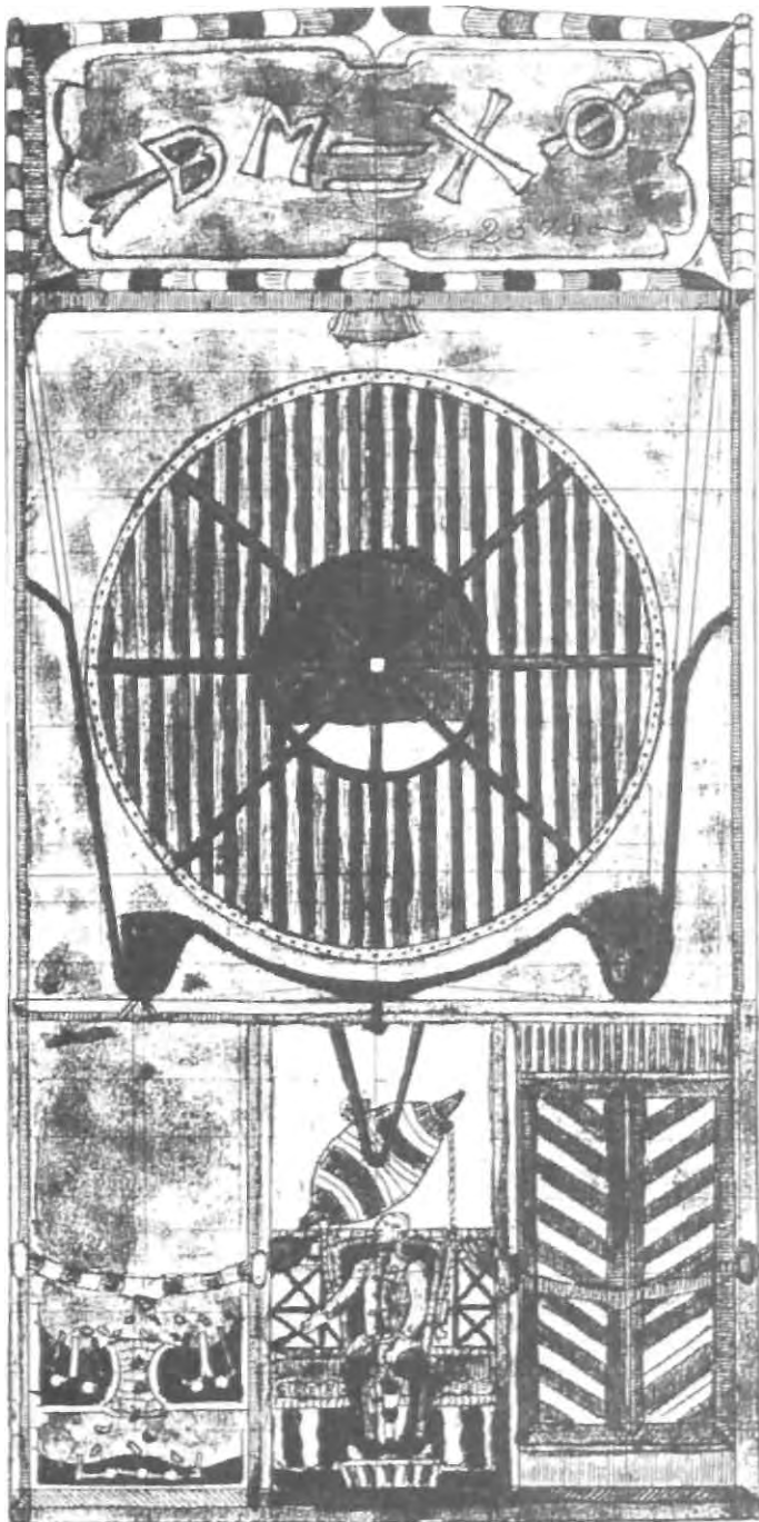
Example of a later design for Dellschau's Airpress Motor (inside view)
