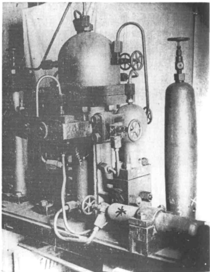
Generator, built between 1881-1885
